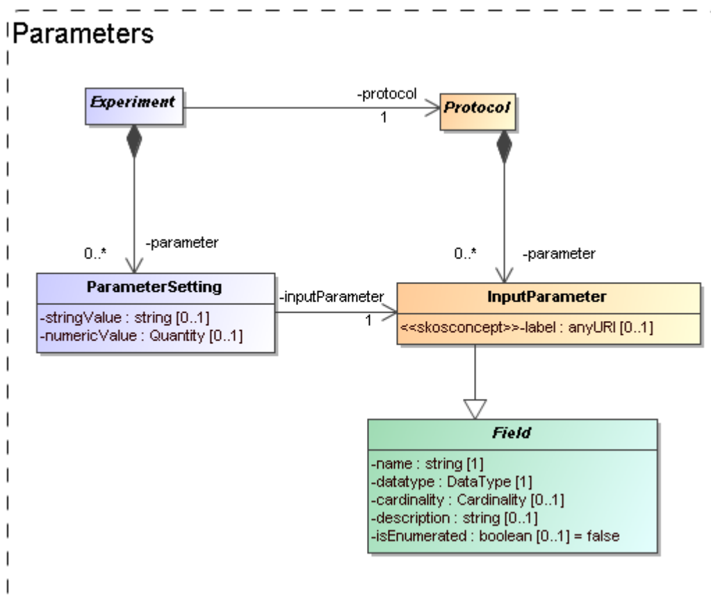
Figure 8: Modelling the parameters: definition under ( experimental ) Protocol, values under Experiment.
