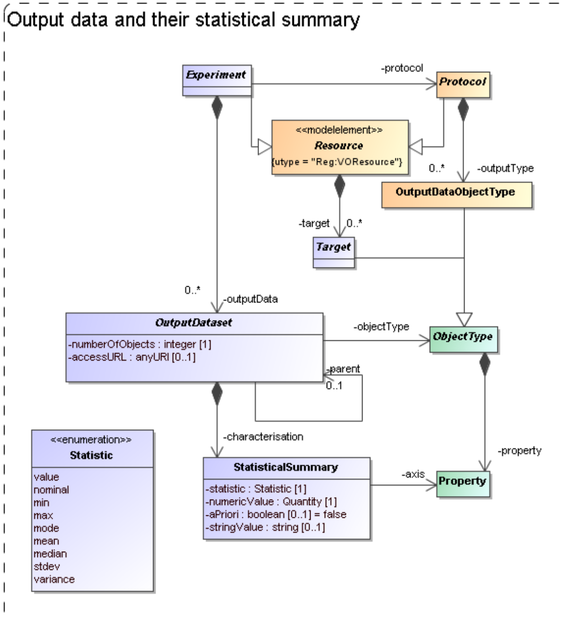
Figure 11: Modelling Output data sets and their contents.
