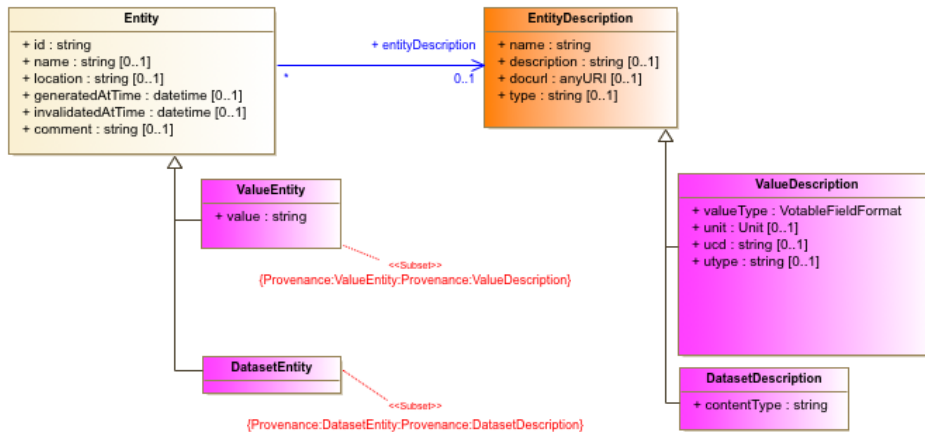
Figure 6: Partial class diagram focused on Specific types of Entity classes.
