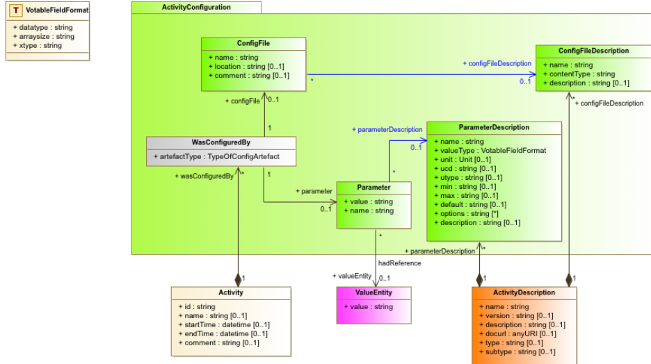
Figure 7: Partial class diagram focused on the ActivityConfiguration package. The Parameter and ConfigFile classes provide configuration information for an Activity instance. The right side of the diagram shows the descriptions, where an ActivityDescription class is bound with the ParameterDescription and ConfigFileDescription classes.
