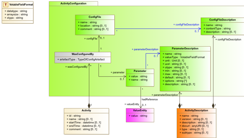
Figure 7: Partial class diagram focused on the ActivityConfiguration package. The Parameter and ConfigFile classes provide configuration information for an Activity instance. The right side of the diagram shows the descriptions, where an ActivityDescription class is bound with the ParameterDescription and ConfigFileDescription classes.
